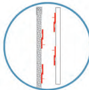
Z-Bar Interlocking Hanging System
